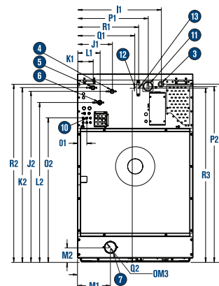
BACK ELEVATION
