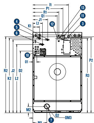
BACK ELEVATION
